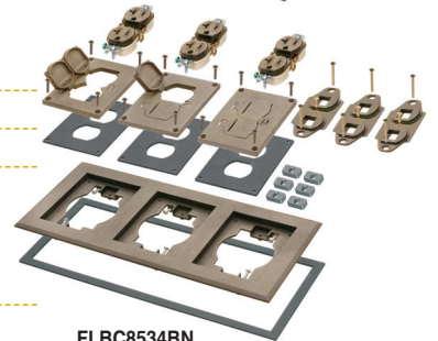
FLBC8534BN Three-gang, Brown
