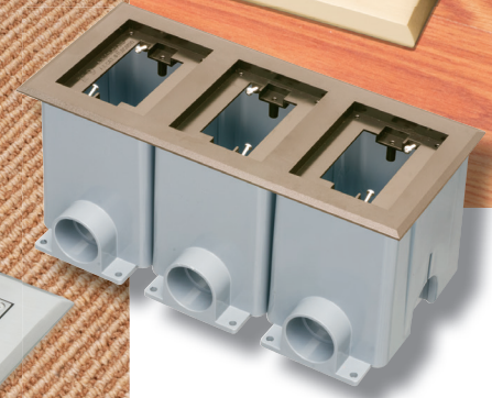
FLBC8535BR PLASTIC cover/frame kit
