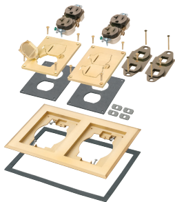
FLBC8524MB Two-gang Brass-plated
