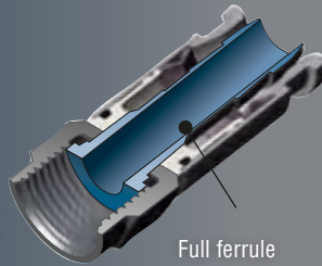
Full ferrule
