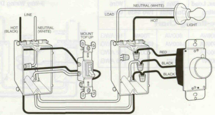
Rotary Dimmer 3-Way Wiring Diagram
