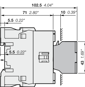
AF12 + CAT4 2-pole auxiliary contact and coil terminal block
