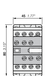
AF12 + CAT4 2-pole auxiliary contact and coil terminal block
