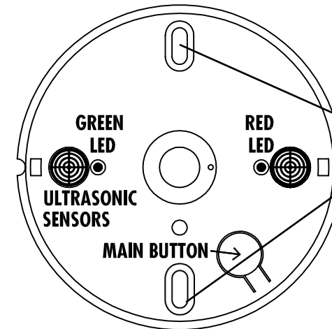
COS-LU DIAGRAM
