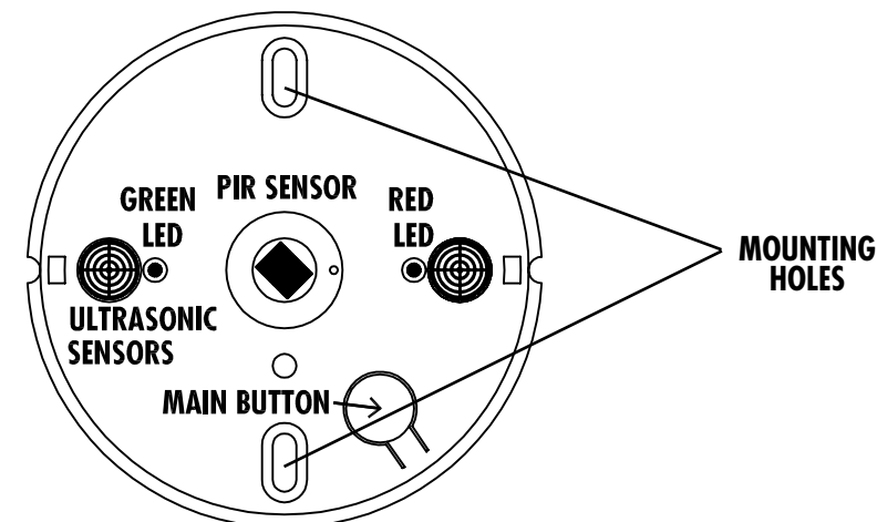
COS-L2T DIAGRAM
