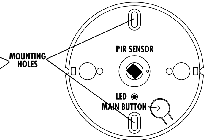
COS-L DIAGRAM
