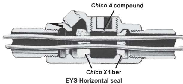
EYS Horizontal seal
