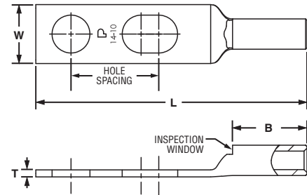
Figure 2: Slotted
