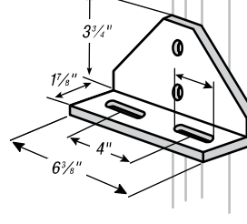
CAT. NO. X204 Slot size is 3/16" x 1 1/2"
