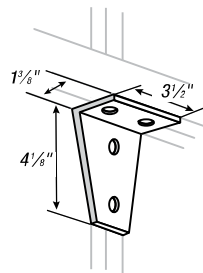
CAT. NO. X289
