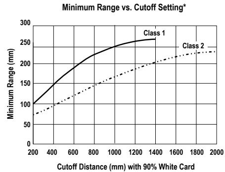
Figure 10. Q60 Minium Range Versus Cutoff Setting
