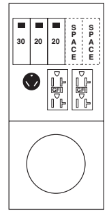
Fig. F R031C010U R32U, (2) 5-20R2GFCI
