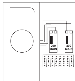
Fig. E RS45508C, RS45508CGP, RS45508CAEP THQD22200WL
