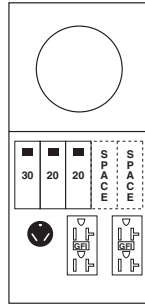
Fig. B M031C010, R031C010 R32U, (2) 5-20R2GFCl
