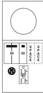
Fig. G M355C010 BR54U, 5-20R2GFCl
