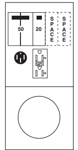
Fig. L M355C010U BR54U, 5-20R2GFCI
