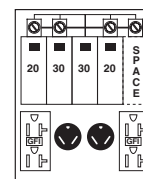
Fig. J U131CTL010 (2) BR32U, (2) 5-20R2GFCI
