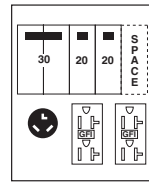
Fig. G U666C010 10-30R, (2) 5-20R2GFCI
