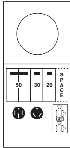
Fig. E M075C010, R075C010 BR54U, BR32U, 5-20R2GFCl
