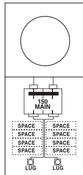
Fig. D R158CR2TLFNG Series
