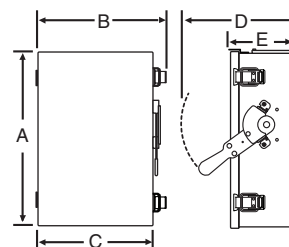
Fig. C General Duty - NEMA Type 3R Side Swing, 200A
