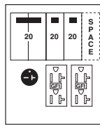
Fig. B U038C010 6-20R, (2) 5-20R2GFCI
