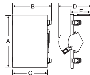
Fig. C Heavy Duty - NEMA Type 3R Side Swing, 200A
