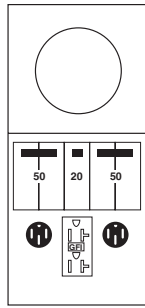
Fig. A M004C010 (2) BR54U, 5-20R2GFCl
