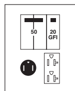
Fig. F U511G 6-50R, 5-20R2
