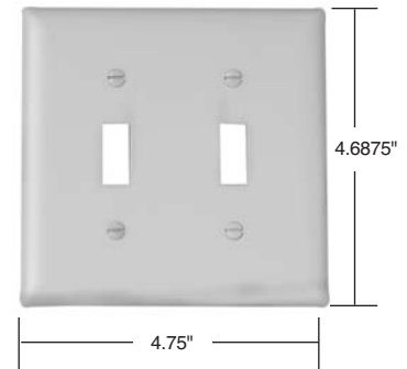
Dimensions for TradeMaster Two Gang
